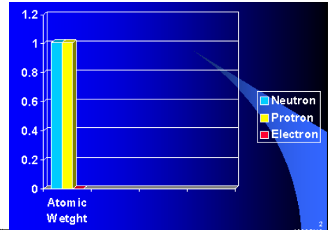
ELECTRON 0.00054858026
